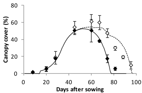
Fig. 7. Simulated (lines) and observed (symbols) green canopy cover for tef under soil fertility stress (T0) in Maiquiha during the season of 2009. Both irrigated (IR, dotted line, open symbol) and rainfed (RF, full line, filled symbol) canopy cover development under soil fertility stress are well simulated. Error bars indicate \pm standard deviation for three replications (n=3).
