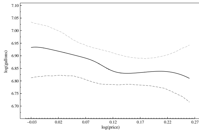
Figure 2: The estimated price component m_p[\log(price_i)] for the PLAM specification in Equation (9) when the RTECS price measure is considered. The estimate is based on the pooled 1991 and 1994 surveys (5260 households). 95% confidence intervals obtained by bootstrap.
