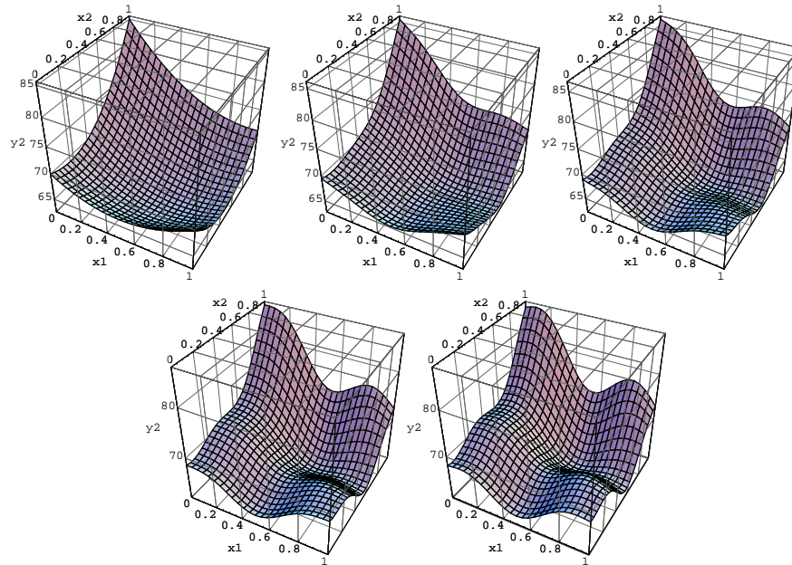
Figure 2: Surfaces for the true mean function of the response y_2 when \gamma = 0.00 (top left), 0.25 (top middle), 0.50 (top right), 0.75 (bottom left), and 1.00 (bottom right), respectively.
