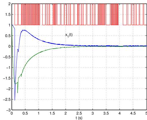
Figure 2. The state and switching signal evolution
