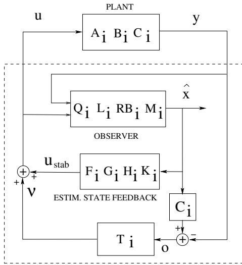
Figure 1. The observer-based compensator structure
