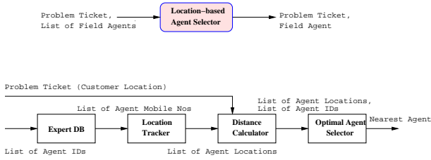
Figure 2: Location-based Agent Selector Service.
