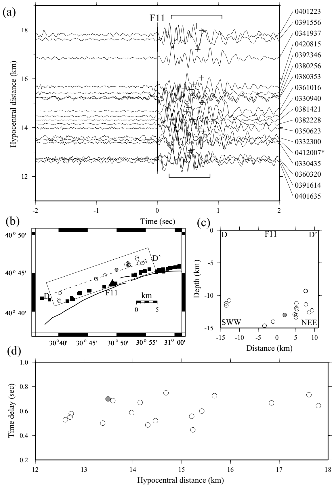
Figure 9. Fault-parallel seismograms at station F11 for events at cross-section DD' parallel to the fault strike. Other symbols and notation are the same as in Fig. 6(a). (b) A location map of the events producing the seismograms shown in (a). (c) Hypocentres projected from the box in (b) along the cross-section DD'. (d) Time differences between S arrivals and centres of trapped waves groups for different hypocentral distances. The waveforms of event 0412007 marked with an asterisk in (a) and grey circles in (b)–(d) are modelled in Fig. 11.
