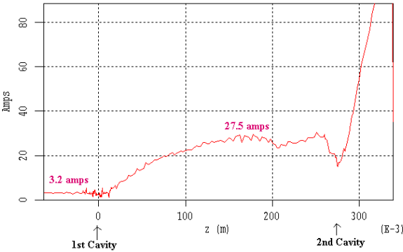
Fig. 7. RF current vs. Z.
