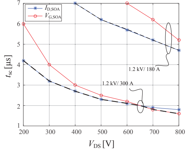
Fig. 11. Short circuit SOA of the two SiC MOSFET power modules based on the two proposed criteria at T = 25^\circ C . I_{D,SOA} - short circuit current-based criterion and V_{G,SOA} - gate voltage-based criterion. Dashed line corresponds with the final SCSOA.
