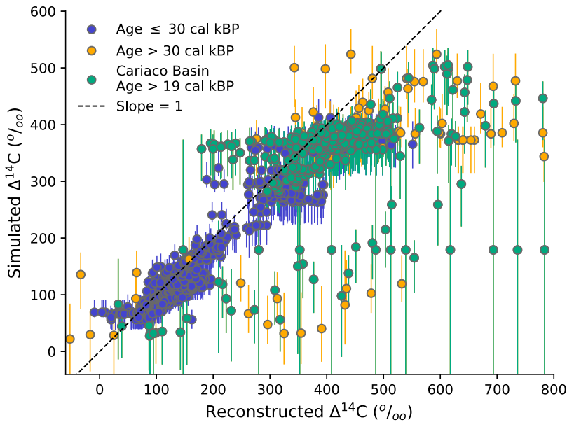
Figure 3 Comparison of simulated and reconstructed marine \Delta^{14}\text{C} for locations which contain records contributing to IntCal20 (Bard et al. 1990, 1998, 2004a, 2004b, 2013; Burr et al. 1998, 2004; Hughen et al. 2000, 2004, 2006; Cutler et al. 2004; Fairbanks et al. 2005; Durand et al. 2013; Heaton et al. 2013). Simulation results are for ocean climate scenario GS forced with the mean atmospheric \Delta^{14}\text{C} record where error bars indicate the combined uncertainty of atmospheric \Delta^{14}\text{C} and scenarios CS and PD. Four data points are not shown (two data points with reconstructed \Delta^{14}\text{C} < -150\text{‰} and simulated \Delta^{14}\text{C} \sim 20\text{‰} , plus two data points with reconstructed \Delta^{14}\text{C} > 1500\text{‰} and simulated \Delta^{14}\text{C} \sim 200\text{‰} ).
