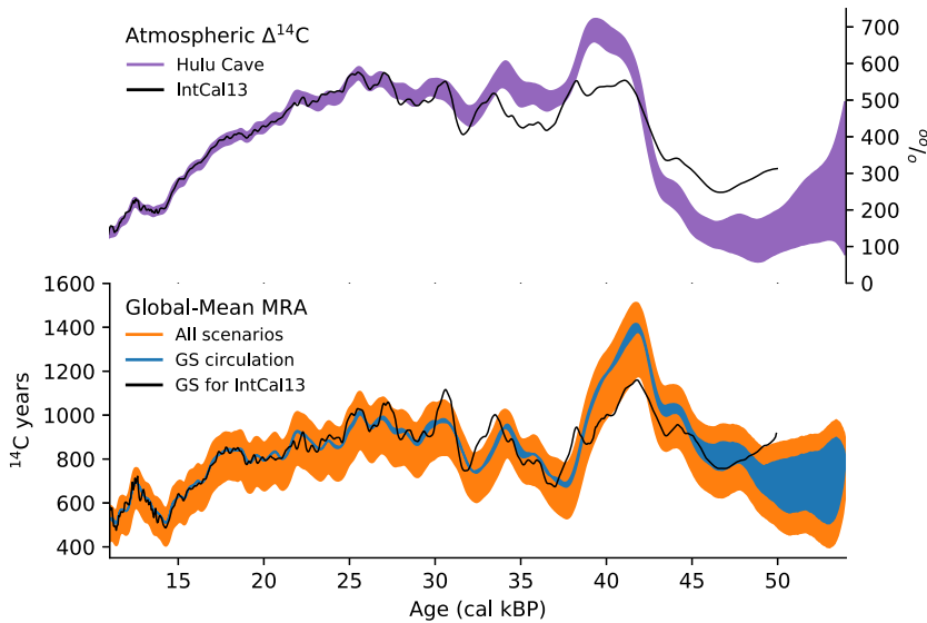
Figure 1 (Top) Atmospheric \Delta^{14}\text{C} from the Hulu Cave record (Southon et al. 2012; Cheng et al. 2018) used as transient forcing in our simulations. Plotted band spans the uncertainty range (mean values \pm 2\sigma ). (Bottom) Simulated global mean marine reservoir ages (MRA) in the upper 50 m, plotted are global averages excluding regions poleward of 50^\circ latitude. Upper and lower bounds of all results are plotted in orange. Scenario GS is plotted in blue. The black lines show previous model results for scenario GS (Butzin et al. 2017) forced with atmospheric \Delta^{14}\text{C} according to IntCal13 (Reimer et al. 2013). (Please see electronic version for color figures.)
