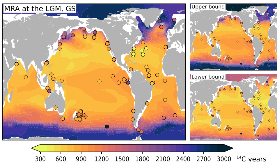
Figure 2 Geographic distribution of simulated marine reservoir ages (MRAs) in the upper 50 m at the Last Glacial Maximum (time average over 19–23 cal kBP). Left: Results for scenario GS forced with the mean atmospheric \Delta^{14}\text{C} record; right: upper and lower bounds of all simulation results involving scenarios CS (top) and PD (bottom). Filled circles are foraminifera-based MRAs compiled by Skinner et al. (2017).
