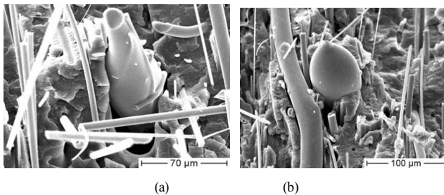
Figure 11. SEM picture of the presence of fiber heads (gravels) in the composite
