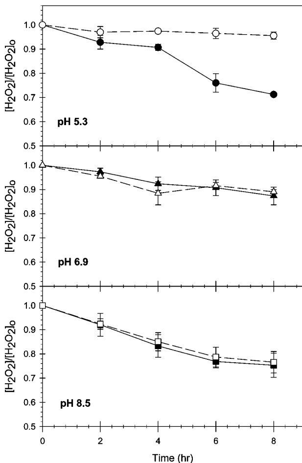
FIGURE 3. H 2 O 2 loss in the FeAlSi-ox/H 2 O 2 system in the absence (solid lines) and presence (dashed lines) of t -BuOH; [phenol] 0 = 0.5 mM; [H 2 O 2 ] = 50 mM; [FeAlSi-ox] = 3 g/L; and [ t -BuOH] = 200 mM.
