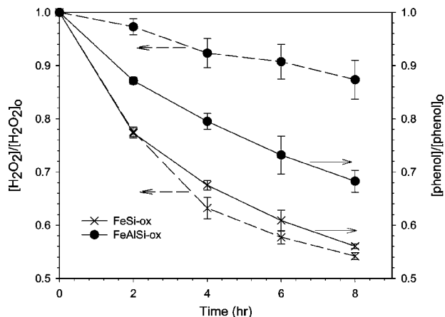
FIGURE 4. Phenol and H 2 O 2 loss in the FeSi-ox/H 2 O 2 and FeAlSi-ox/H 2 O 2 systems; [phenol] 0 = 0.5 mM; [H 2 O 2 ] = 50 mM; [FeAlSi-ox] = [FeSi-ox] = 3 g/L; and pH 6.9. The pH decreased by less than 0.3 units during the reaction.
