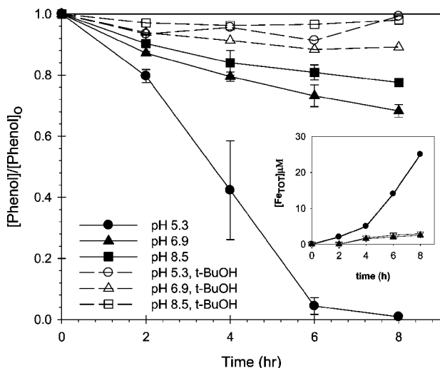
FIGURE 2. Effect of pH on phenol loss in the FeAlSi-ox/H 2 O 2 system in the absence (solid lines) and presence (dashed lines) of t -BuOH; [phenol] 0 = 0.5 mM; [H 2 O 2 ] = 50 mM; [FeAlSi-ox] = 3 g/L; and [ t -BuOH] = 200 mM. [Fe TOT ] as a function of time (inset): (●) pH 5.3; (▽) pH 6.9; (▲) pH 8.5. For the purpose of clarity, error bars were eliminated from the data in the inset. In all cases, pH decreased by less than 1 unit during the reaction.
