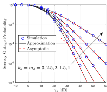
Fig. 3. P_{\text{sop}} versus \bar{\gamma}_d for m_e = k_e = 2 , \bar{\gamma}_e = 5 dB, and R_s = 1 .
