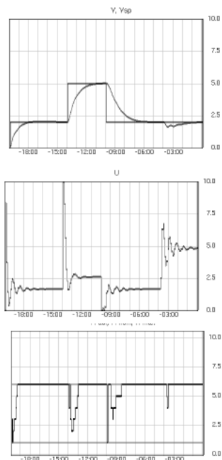
Fig. 7 PID control of the lower tank. h_{max} = 6s
