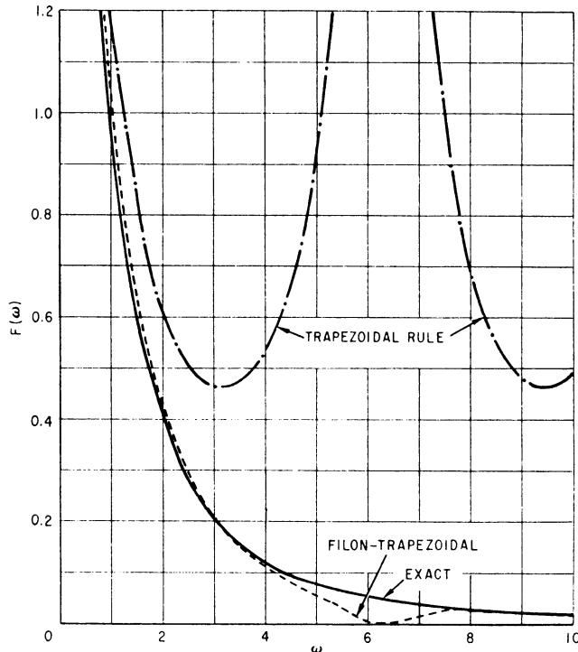
FIG. 1. Exact and approximate values for the Fourier integral F(\omega) = \int_{-\infty}^{\infty} dt \exp(-|t| + i\omega t)
