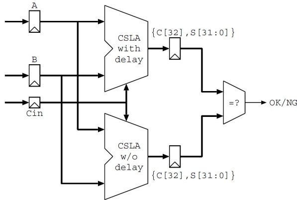
Figure 7: Evaluation Circuit
