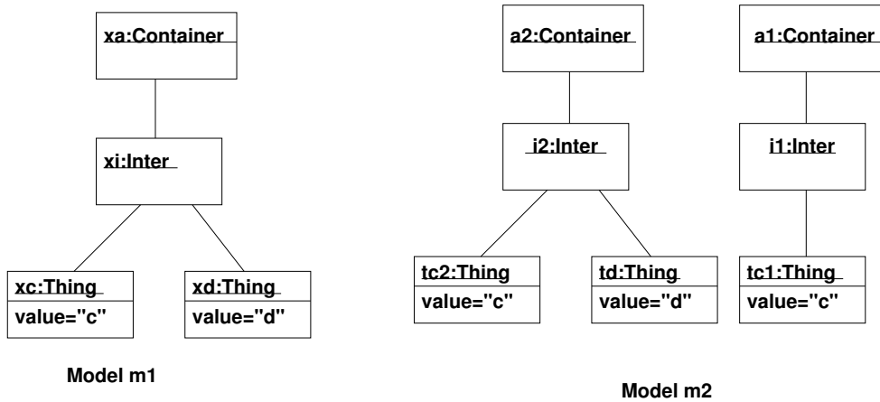
Figure 9: m_1 and m_2 are (two-way) consistent according to QVT-R transformation \text{Sim} , but no set of bidirectional trace objects can link them
