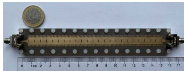
FIGURE 7. Fabricated BCSIW LWA prototype.
