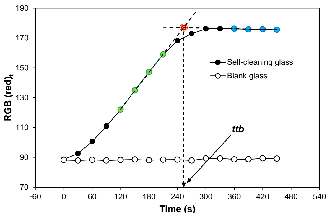
Fig. 2. – (a) A series of images recorded at 30 second irradiation intervals for two glass samples, namely; self-cleaning glass (top) and, plain glass (bottom). (b) A plot of variation of the \text{RGB (red)}_t with irradiation time, extracted from the images shown in (a). \text{RGB (red)}_t is the value of the RGB
