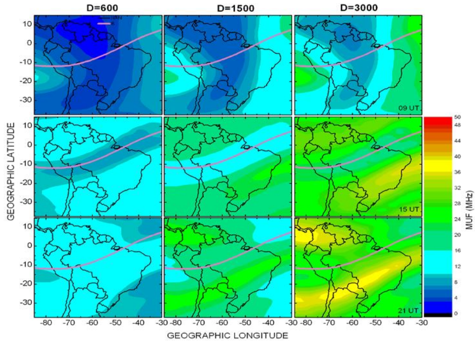
Figure 5: Maps of MUF calculated with foE, foF2 and hmF2 from PARIM for solar minimum conditions.
