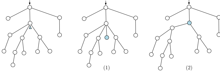
Fig. 3: Rémy’s procedure gives two ways to obtain a plane tree with n edges and a marked vertex v from a plane tree with n - 1 edges and a marked corner: (1) in the first way v is a leaf, (2) in the second way v is a non-leaf.
