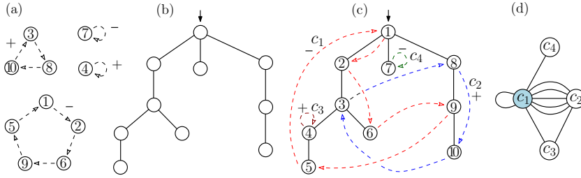
Fig. 1: (a) A C-permutation \sigma . (b) A plane tree T . (c) The C-decorated tree (T, \sigma) . (d) The underlying graph of (T, \sigma) .
