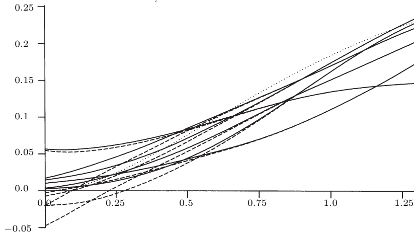
Figure 1. Six pairs of density estimates based on random samples of size 50 from the Gamma (3,1) distribution, L(u) = uK(u) , K the biweight kernel, and h = 1.3 . Solid lines: \hat{f}_P , dashed lines: \hat{f} , dotted curve: f . The boundary region 0 < x < h only is shown.
