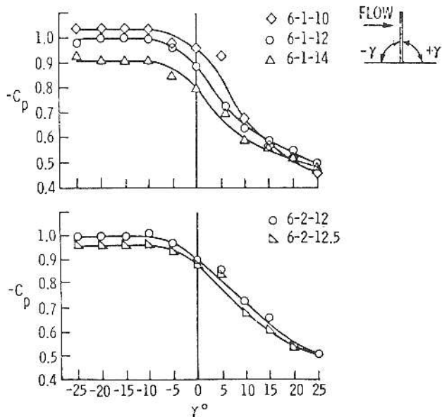
Figure 6. Variation of CP with sweep.
