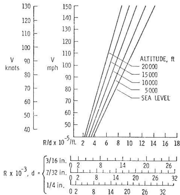
Figure 3. Reynolds numbers for various cylinder diameters.
