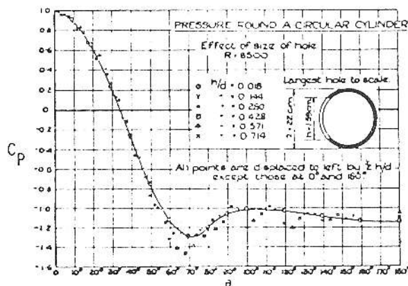
Figure 8. Effect of hole size on pressure coefficients (Ref. 8).
