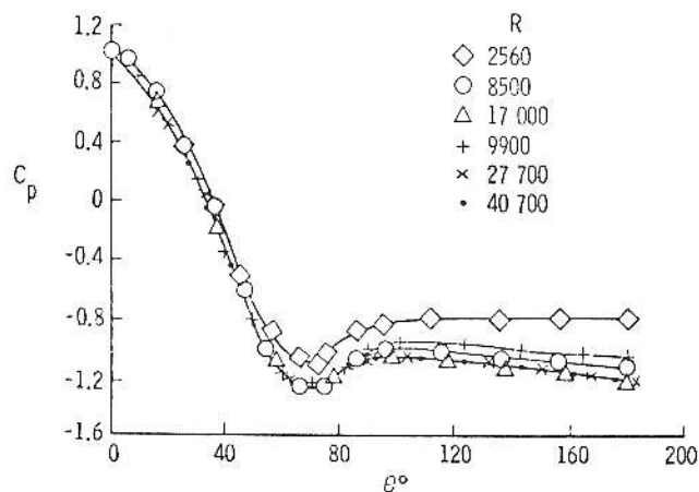
Figure 2. Typical pressure distributions on two-dimensional cylinders (Refs. 10 and 14).
