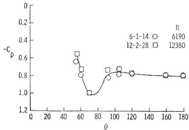
Figure 9. Effect of Reynolds number on pressure coefficient.
