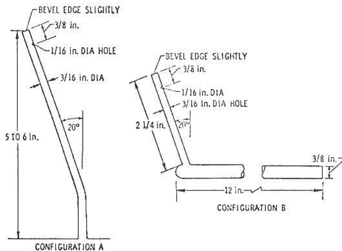
Figure 10. Two examples of total energy sensors tested.
