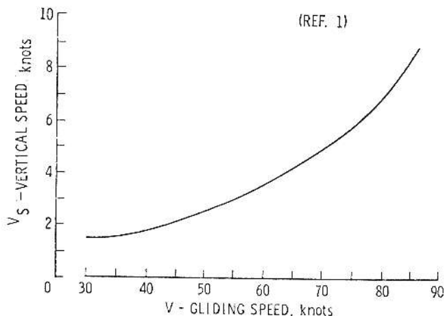
Figure 1. Typical polar: SGS 1-26 (Ref. 1).
