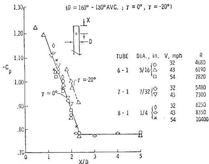
Figure 7. Pressure coefficients as a function of hole position.
