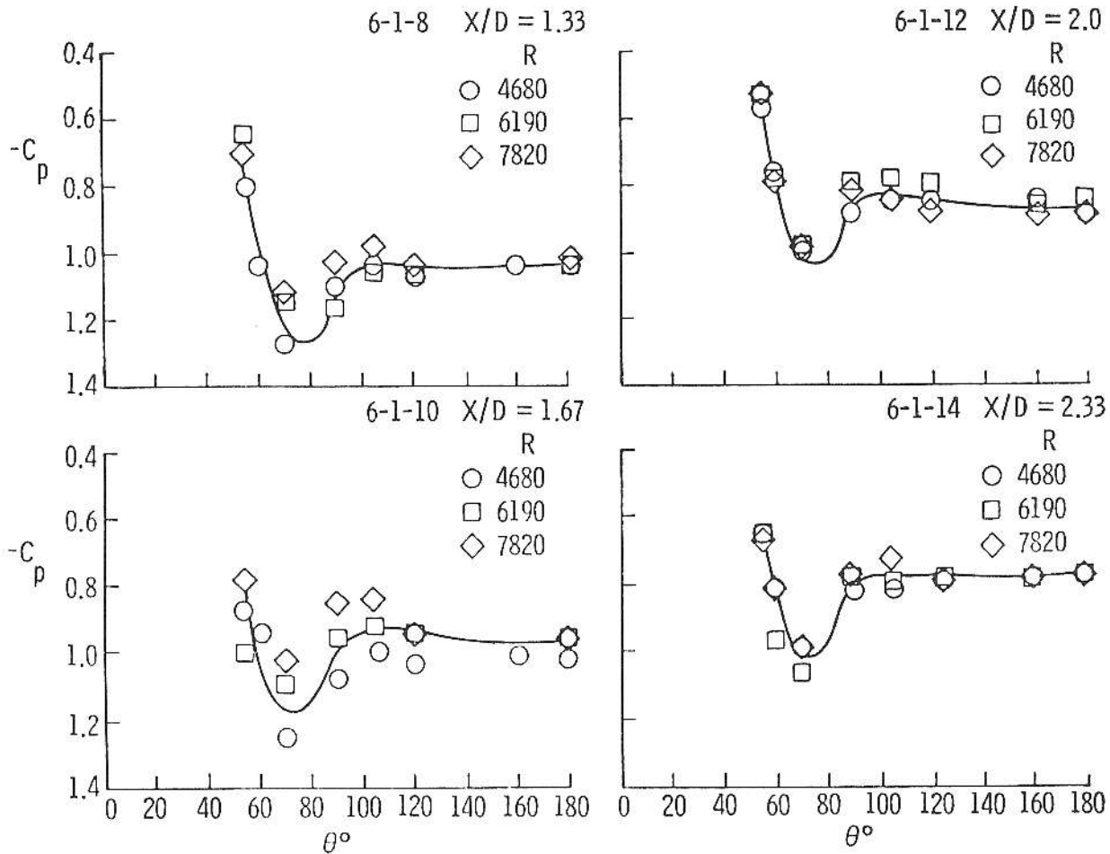
Figure 5. Typical pressure distributions on three-dimensional cylinders.
