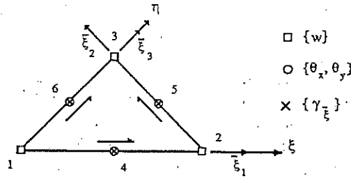
Figure 2. Geometric description and nodal variables of the TLLL plate element
