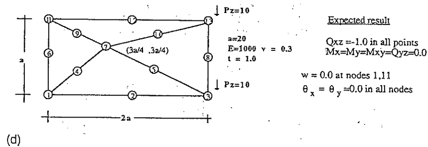
Figure 4. Patch tests for the TLL element: (a) constant bending moment test; (b) cantilever plate under constant bending moment; (c) square plate supported at three corners under point load and (d) constant shear patch test
