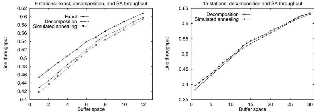
Figure 4: Computed throughput of simulated annealing compared with full and reduced enumerations for 9 stations (left); compared with reduced enumeration for 15 stations (right).
