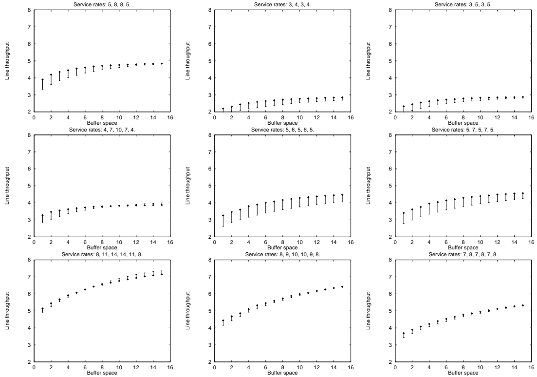
Figure 5: Simulated annealing with decomposition evaluation (dash ticks) versus enumerated Markovian (dot ticks) throughputs for unbalanced lines with 4–6 stations.
