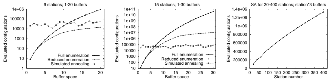
Figure 6: Performance of simulated annealing compared with full and reduced enumerations for 9 stations (left); compared with reduced enumeration for 15 stations (middle); run for up to 400 stations (right). Note the \log_{10} scale on the ordinate axis.
