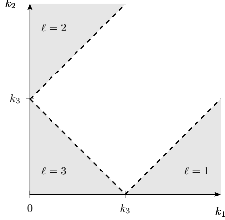
Figure 3: The constraints on the parameters k_j in Corollary 3.2 — if k_1, k_2 take values in the shaded regions then (21) holds with the indicated choice of \ell
