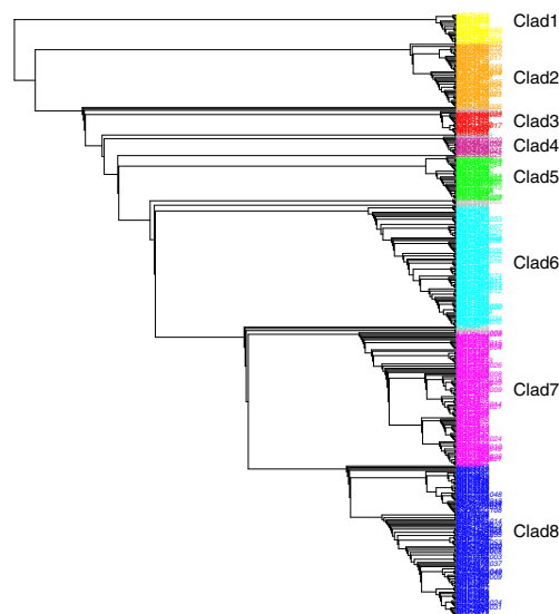
Fig. 3. Most parsimonious tree found with cladistics with the identification of the eight groups and their corresponding colours.
