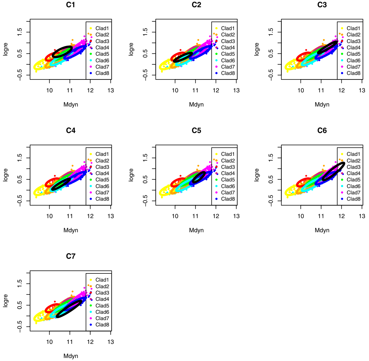
Fig. C.4. Comparison of the positions of the groups found in Fraix-Burnet et al. (2010) and those of the present paper, as projected onto the \log r_e vs. M_{\text{dyn}} diagram. The colour-coded ellipses are the inertia ellipses for each group from the present paper, and the black ellipse is the one for the group from Fraix-Burnet et al. (2010) indicated on top each graph. See also Fig. 9.
