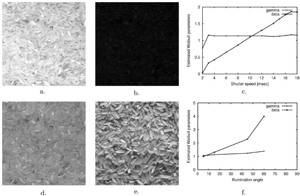
Figure 3. Weibull parameters as function of illumination intensity a–c and illumination angle d–f. a. shows the rice image at 18 msec shutter speed, saturating the white portions of the image. b. shows the rice image at 3 msec shutter speed, saturating the dark portions of the image. The Weibull parameters as function of shutter speed are illustrated in c. Within the dynamic range of the camera, the \beta -parameter is clearly linear with intensity. d. shows the rice image with frontal illumination, whereas e shows oblique illumination. Note the large variation in Weibull parameters, shown in f.
