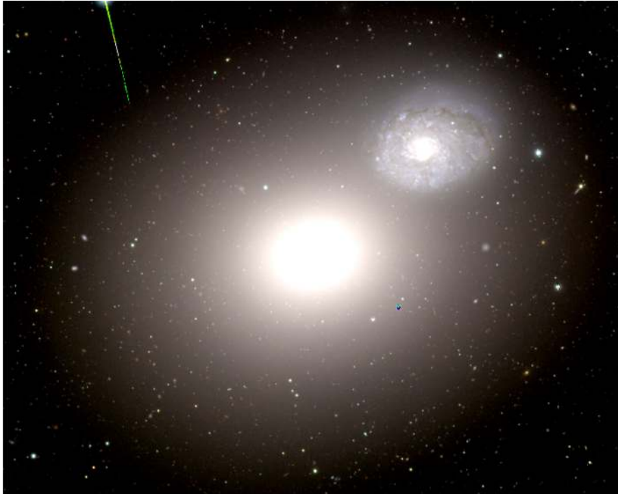
Figure 18. Subaru/Suprime-Cam gri colour image of NGC 4649 (left) and NGC 4647 (right). The projected separation between the two galaxies is 13 kpc. There are no clear signs of interaction between the two galaxies. North is up, east is left.
