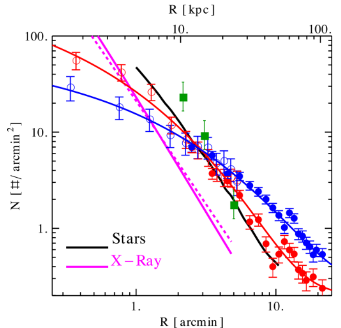
Figure 4. GC surface density profiles. Blue and red GCs are colour coded accordingly. Open and filled circles are from HST /ACS and from ground-based photometry, respectively. The two solid lines are the best fits to equation (1). Green squares are PNe data. The black line is the arbitrarily renormalized stellar surface brightness profile of NGC 4649 in the V band from Kormendy et al. (2009). The magenta thick and dashed lines are the outer slope of the X-ray surface brightness profile from ROSAT and from Chandra , respectively. The red GCs are more centrally concentrated than the blue GCs.
