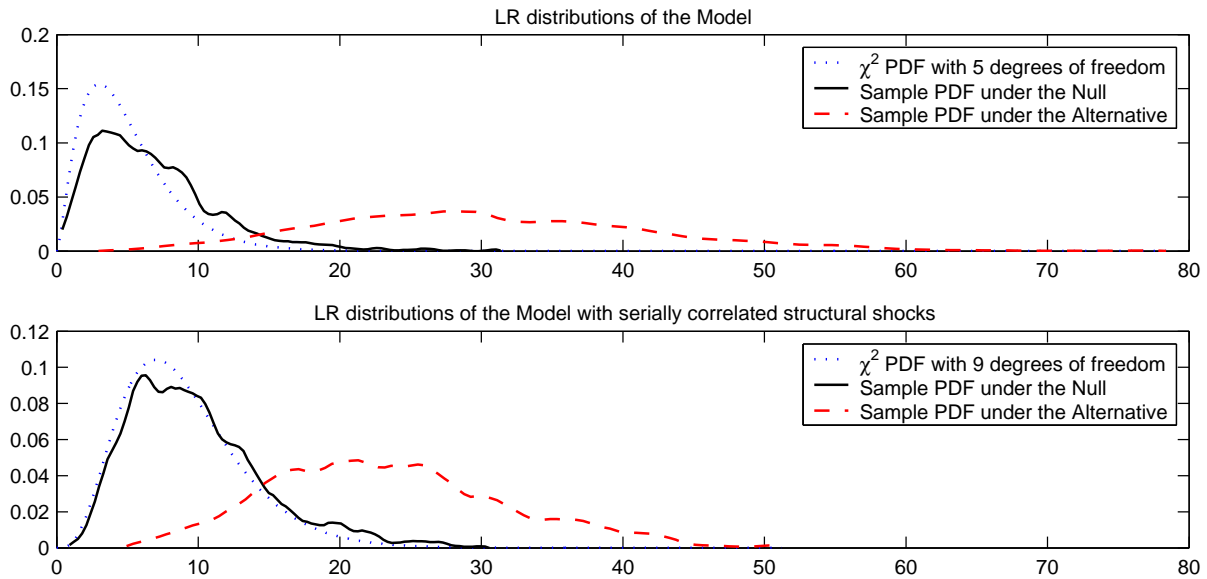
Figure 3: Empirical Distribution of the Likelihood Ratio
