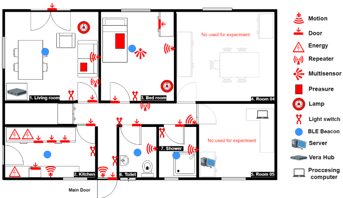
Figure 2. Smart Spaces Lab Layout
