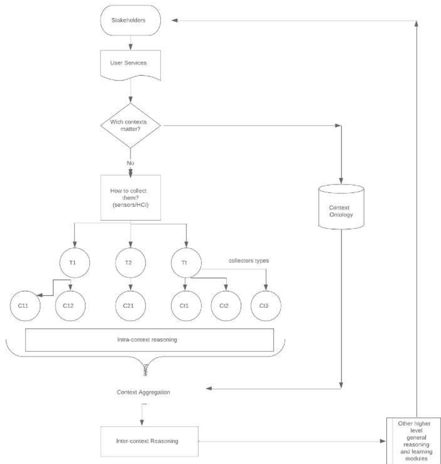
Figure 4. Context-awareness Architecture
