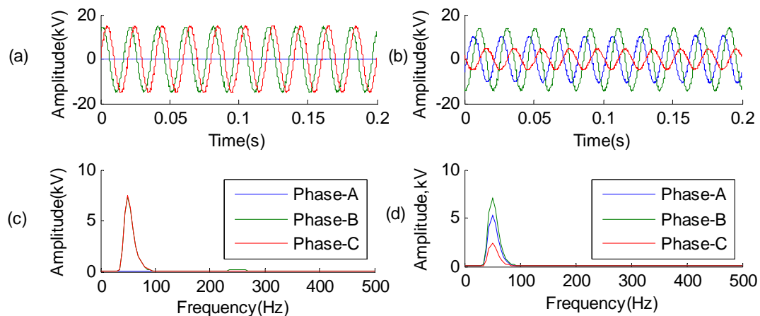
Figure 5. (a) Single phase-to-ground voltage; (b) Fundamental ferroresonance; (c) Mean amplitude curve of single phase-to-ground voltage; (d) Mean amplitude curve of fundamental ferroresonance.
