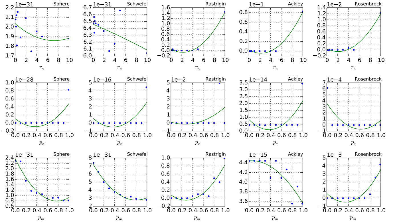
Figure 1: Parameter test results on r_a , p_c , and p_m .
