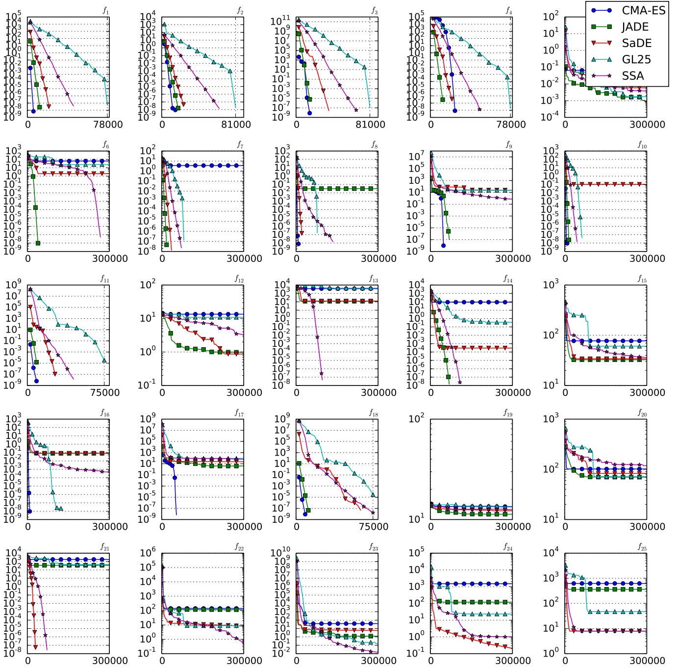
Figure 3: Median convergence test results.
