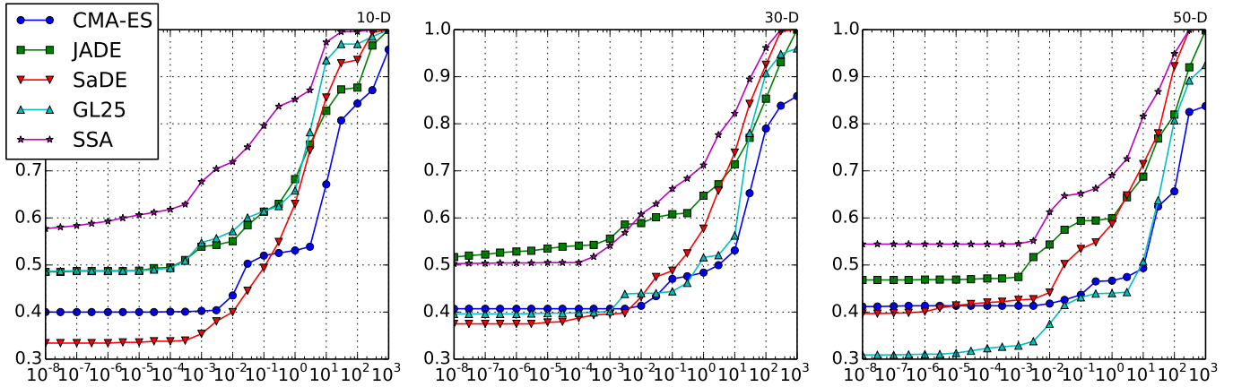
Figure 4: Empirical cumulative distribution of success rate test results.
