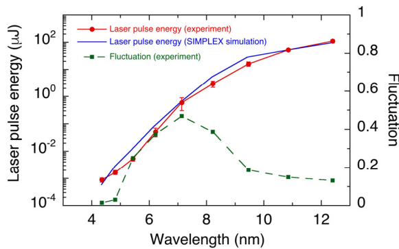
Figure 5: FEL gain curve of the SACLA-BL1. The radiation wavelength was scanned by means of changing the undulator's K-value.
