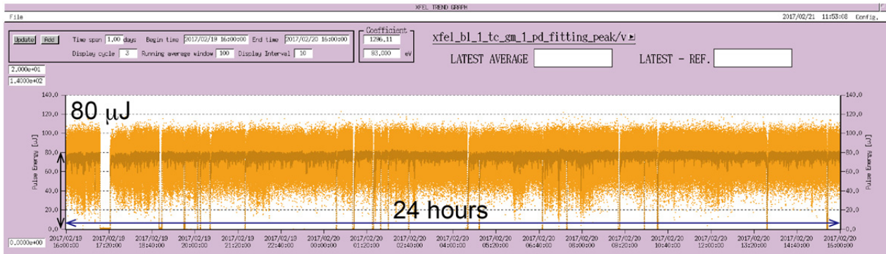
Figure 4: Trend graph of laser pulse energy at a 93-eV photon energy in 24 hours. The orange and brown dots indicate single shots and 100-shot-averaged, respectively. Stable laser pulses are delivered to experimental users for a long time.
