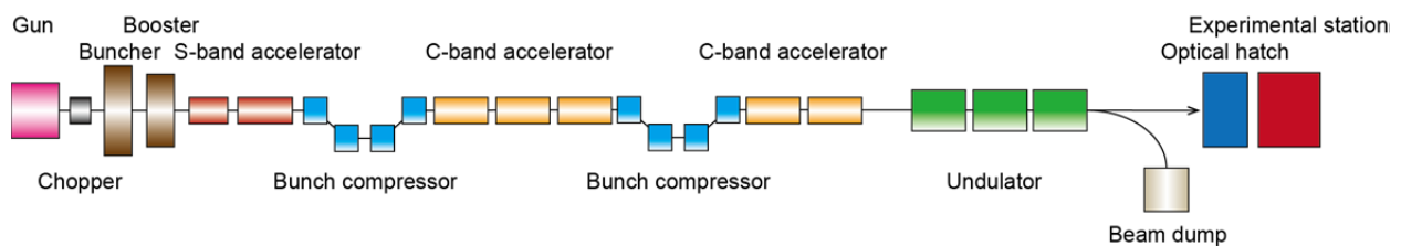
Figure 1: Layout of the soft XFEL beamline of SACLA.
