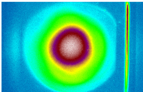
Figure 3: Spatial profile of the 100-eV soft XFEL beam. The horizontal full screen size is 17 mm.
