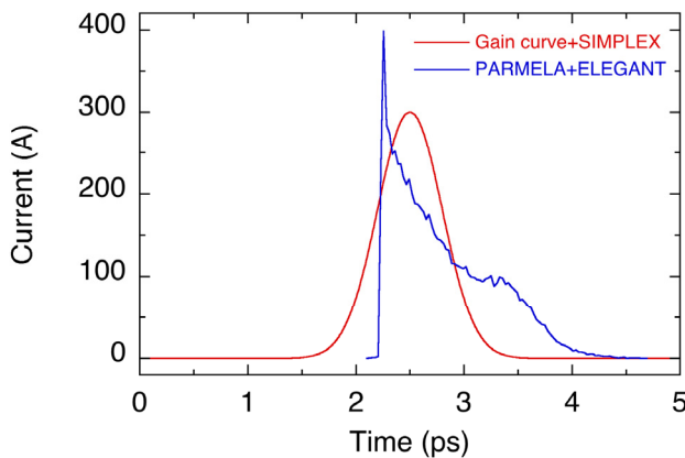
Figure 6: Electron current profiles at the undulator line obtained by the SIMPLEX and the PARMELA-ELEGANT simulations.
