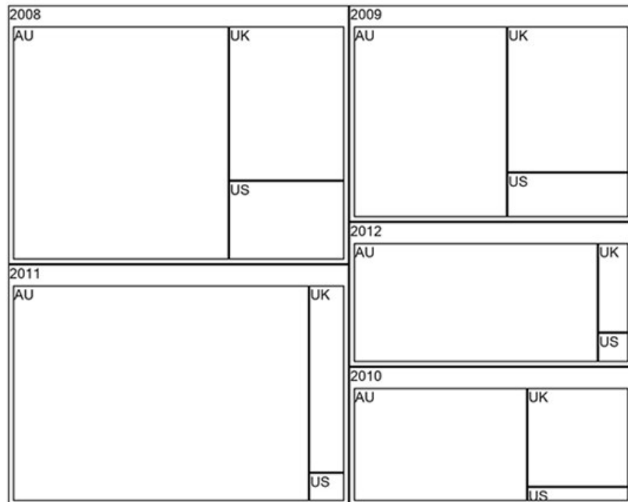
Attribute values compared by attribute value combinations
