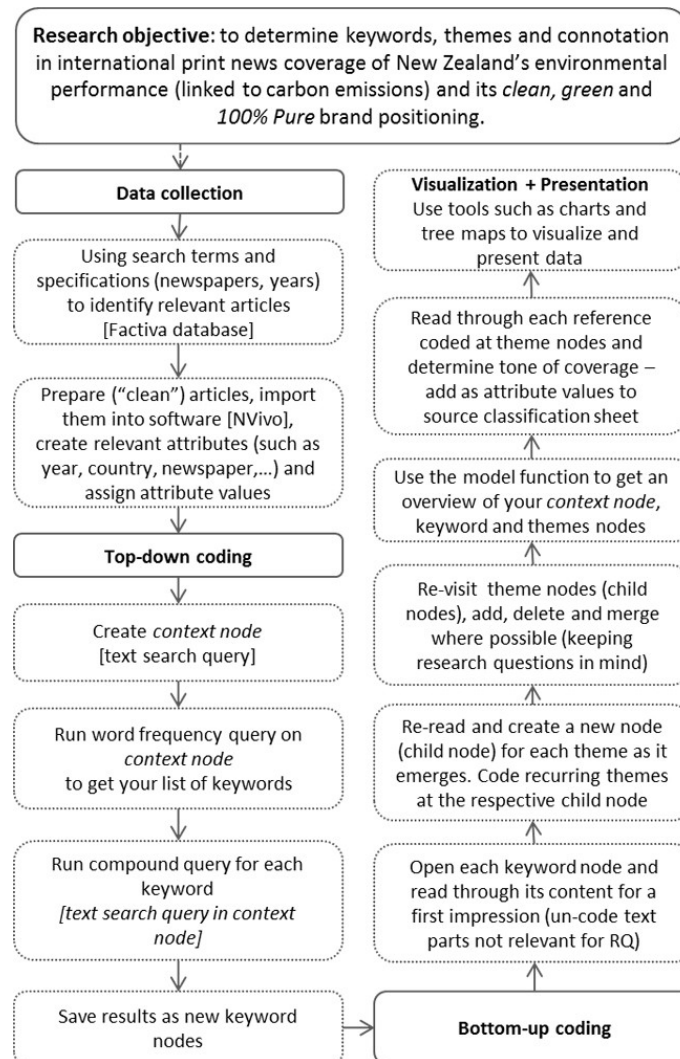
Figure 1: QDAS-assisted multi-level coding approach to qualitative content analysis of news articles [39]
