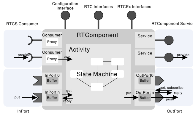
Fig. 1. The proposed architecture of RT-Component model. The RT-Component has a component body, common interface for metadata acquisition, component action, data ports, service ports and configuration interface.
