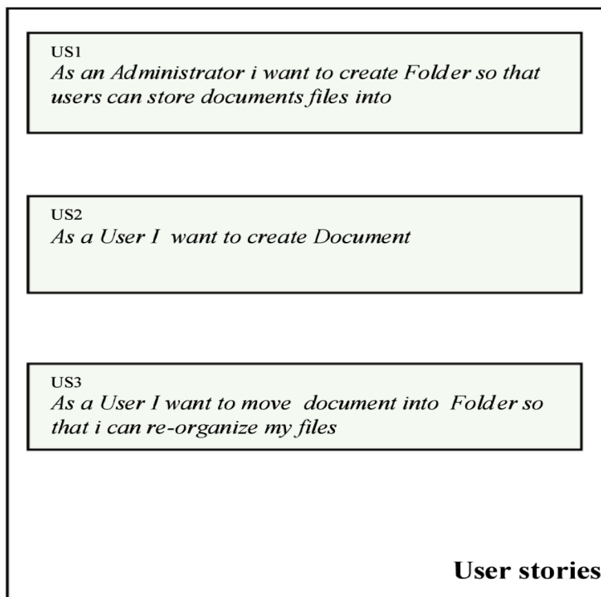
Figure 2. User stories
