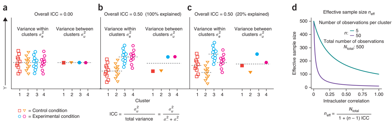
Figure 2 Graphs illustrating why clustering affects the type I error rate. ( a–c ) Graphical representation of three data sets with overall intracluster correlations ICC of 0.00 ( a ), 0.50 ( b ), fully explained by experimental condition, and 0.50 ( c ), partly explained by experimental condition, respectively. The ICC is calculated from the variance between clusters (inferred from the deviations of the cluster means from the grand mean, represented by the horizontal dashed line) and the total variance (that is, the sum of the variance between clusters and the variance within clusters, calculated from the deviations of individual observations from their cluster mean). ( d ) Effective sample size as function of the ICC under two conditions (number of observations per clusters was 5 or 50, total number of observations was always 500). The higher the unexplained ICC, the larger the difference between the observed sample size ( N_{\text{total}} = 500 ) and the effective sample size. The difference between the observed and effective sample size increases faster when the number of observations per cluster is higher.
