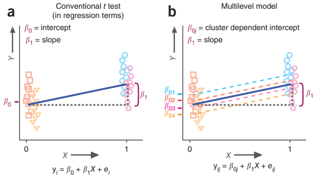
Figure 3 Graphical representations of conventional t test and multilevel analysis. (a) Graphical representation of the conventional t test in regression terms: the individual observations y_i are a function of the mean of the control group (that is, the intercept \beta_0 ) and, when applicable, the estimated deviation from this mean for observations from the experimental group (that is, the slope \beta_1 ), and an individual error term e_i . X is essentially a weight variable that takes on values 0 and 1 for observations from the control and experimental group, respectively. (b) Graphical representation of multilevel analysis. The individual outcomes of observation i from cluster j , y_{ij} , are a function of the cluster-specific intercept \beta_{0j} plus, when applicable, the estimated deviation from this intercept for clusters belonging to the experimental group, \beta_1 , and an individual-specific error term e_{ij} . The higher the unexplained ICC, the more variation there is in the cluster specific intercepts \beta_{0j} .
