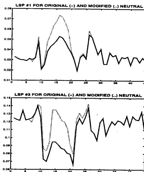
Figure 6: Plots for LSP # 1 (TOP) and LSP # 3 (BOTTOM) of the word break under original neutral (solid) and perturbed to resemble angry conditions (dashed).
