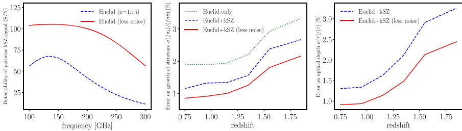
Fig. 3 Left: expected signal-to-noise ratios of the pairwise kSZ signal as a function of frequency. Middle: expected errors on the growth rate as a function of redshift. Right: expected errors on the optical depth as a function of redshift. The “less noise” cases shown in these panels correspond to a factor 10 reduction in the residual noise due to the cosmic infrared background (CIB), which is dominant at small angular scales
