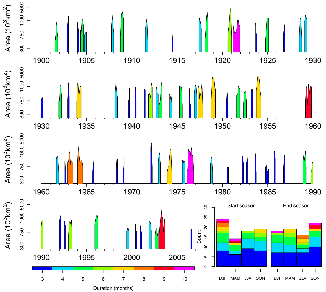
Figure 6: Time evolution of the geographical cross-sectional areas of the 75 droughts events defined by R_{lon} = R_{lat} = 0 with the SPI_3 threshold \leq -1 and lasting for at least 3 months. The histograms (inset) show the seasonal distribution of the dates in which the droughts begin and end. The counts are stacked by event duration.
