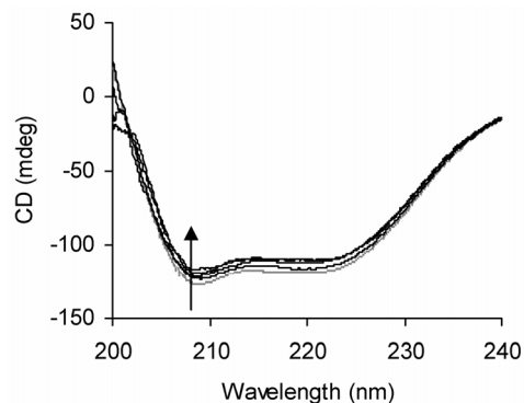
Figure 5. CD spectra of free BSA (dotted line) and complexed (solid lines) with naringin ([BSA]:[naringin] ratios are 1:2, 1:4, 1:6 and 1:8) in 20 mM phosphate buffer of pH 7.0.
