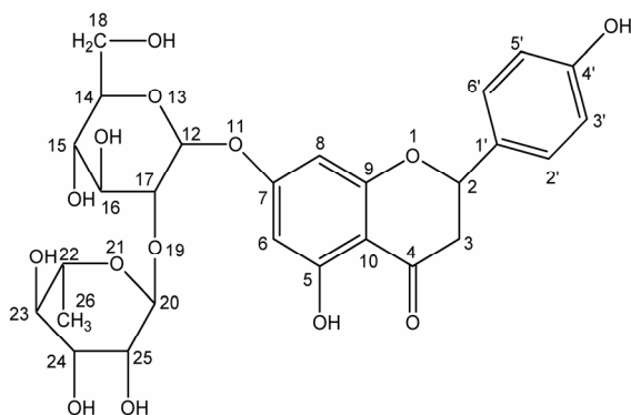
Figure 1. Structure of naringin.
