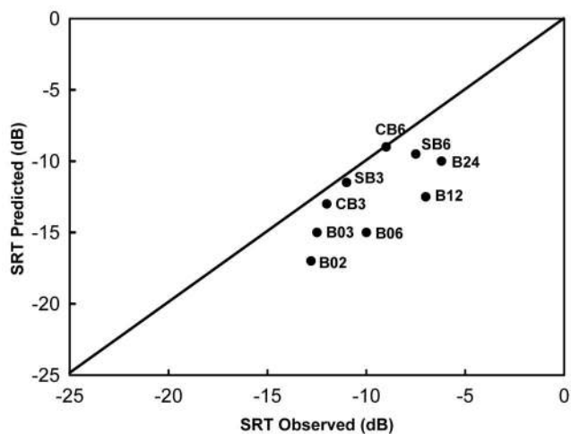
FIG. 10. The SRT (dB) predicted with the extended SII model is plotted as a function of the observed SRT (dB) for the noise maskers used in Festen (1993). Conditions are denoted by abbreviations in the figure. In conditions B02 through B24, conditions consisted of speech fragments that were manipulated by shifting individual frequency bands of the noise masker independently over time. In conditions CB3, CB6, SB3, and SB6, half of the speech masker was replaced by stationary speech noise. For further details the reader is referred to the main text.
