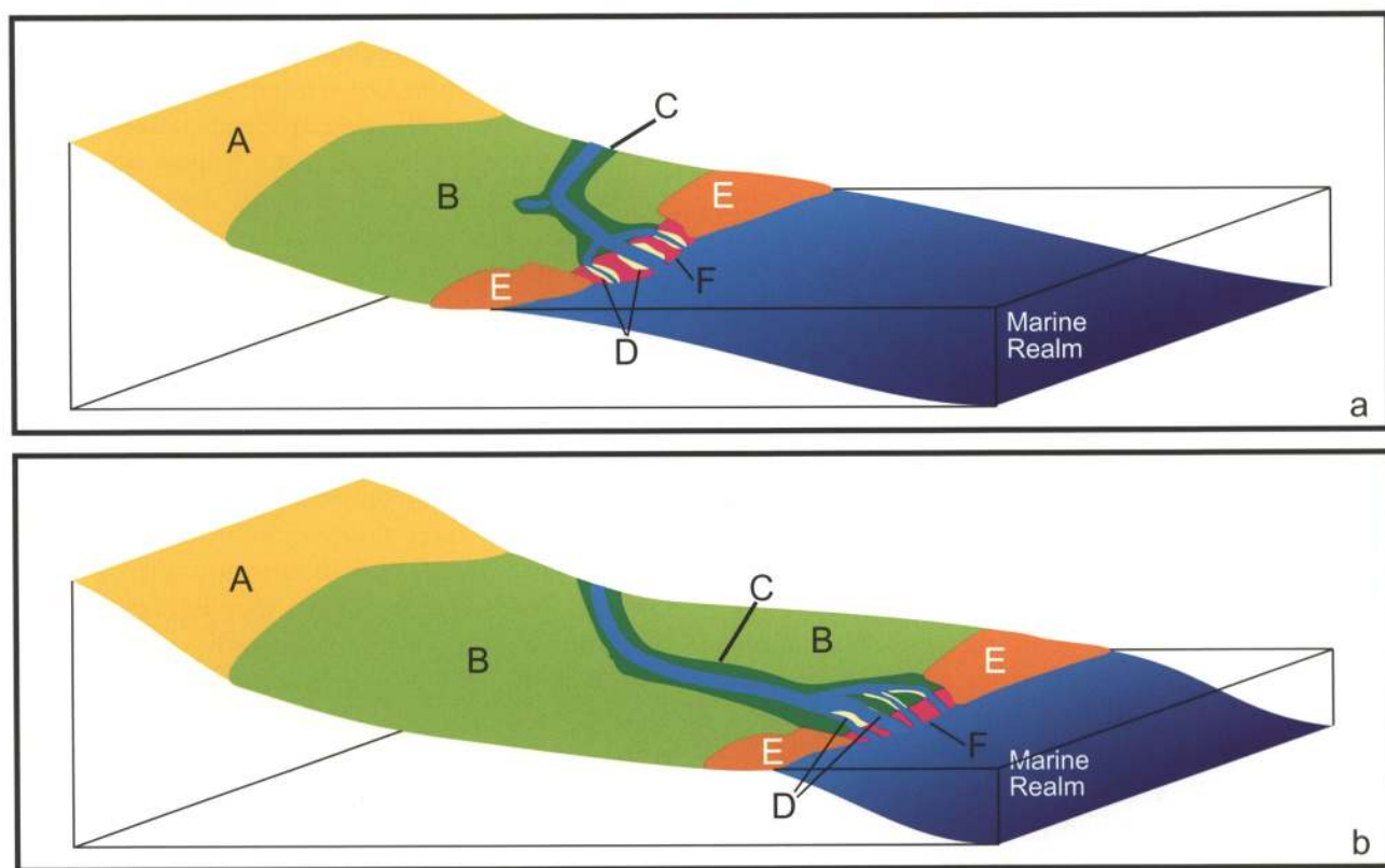
Fig. 2. Schematic representation of the spatial distribution of the SEG. The upper figure (a) depicts the situation during a sea-level high, the lower figure (b) during a sea-level low. A = Upland, B = Lowland, C = River, D = Pioneer, E = Coastal and F = Tidally-influenced SEG.
