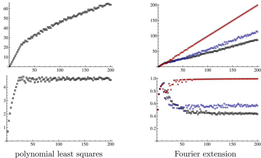
Figure 2: Top row: The parameter n against m = 1, \dots, 200 , where n is chosen as large as possible so that \kappa'_{\text{FE}} \leq 10 for the Fourier extension and \kappa_{\text{PLS}} \leq 10 for polynomial least squares. In the right column, squares, circles and crosses correspond to the parameter values T = \frac{3}{2}, 2, 4 respectively. Bottom row: the scaled parameter n/\sqrt{m} (left) and n/m (right).
