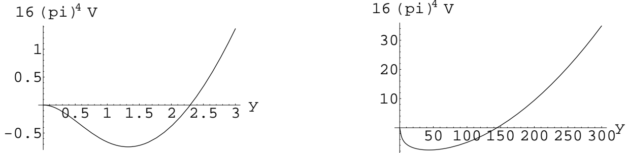
Fig.5: Potential for \tilde{L} = 10, 10000 .
