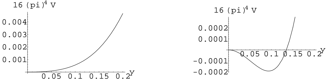
Fig.4: Potential for \tilde{L} = 2.6, 2.7 .
