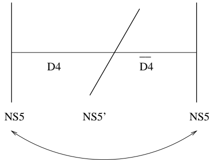
Fig.2: Adjacent D4 and \overline{\text{D4}} between rotated branes.
