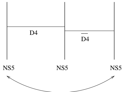
Fig.1: Adjacent D4 and \overline{D4} between parallel branes.
