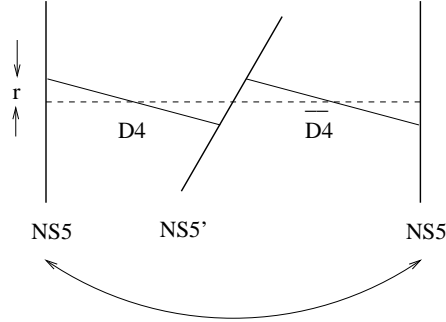
Fig.3: Equilibrium configuration after displacement of 4-branes.
