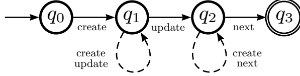
Fig. 6. Automaton from Figure 2 with loops due to Kleene-* sub-expressions removed. Allocation sites e1 , e2 and e3 would collapse, and so the analysis would have to assume that all three enumerations might actually be one and the same, penalizing the opportunities for shadow removal.
