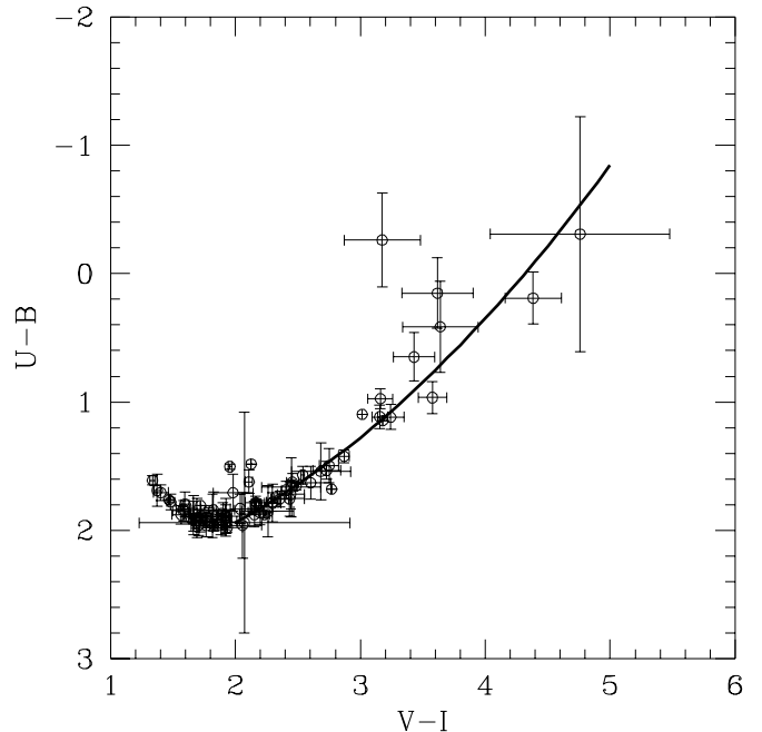
Fig. 4. Adopted (U - B) - (V - I) two-color calibration sequence for cool giants. Symbols represent the same as in Fig. 3. The solid line is a quadratic fit to the data for V - I \geq 2
