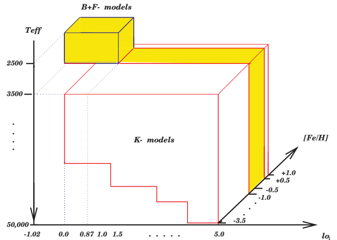
Fig. 19. The (T_{\text{eff}}, \log g, [M/H]) parameter space covered by the present unified library. Solid lines delineate approximate boundaries of available models. (B + F)-models for M-giants are confined to the metallicity range -1.0 \leq [M/H] \leq +0.5 (grey part)
