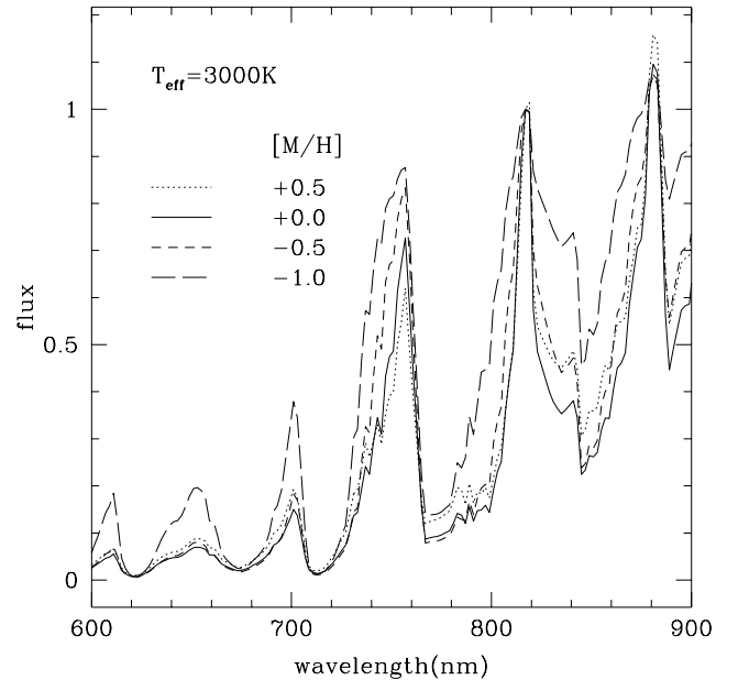
Fig. 2. B-library giant model spectra ( \log g = -0.29 ) for a range in metallicity. All the spectra are normalized at \lambda = 817 nm
