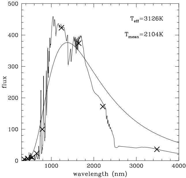
Fig. 8. Black-body fit of temperature T_{\text{mean}} to a synthetic spectrum for T_{\text{eff}} = 3126 K, illustrating the least-squares solution of Eqs. (3). The crosses represent the integrated (heterochromatic) fluxes of the synthetic spectrum measured in the different (broad) bandpasses
