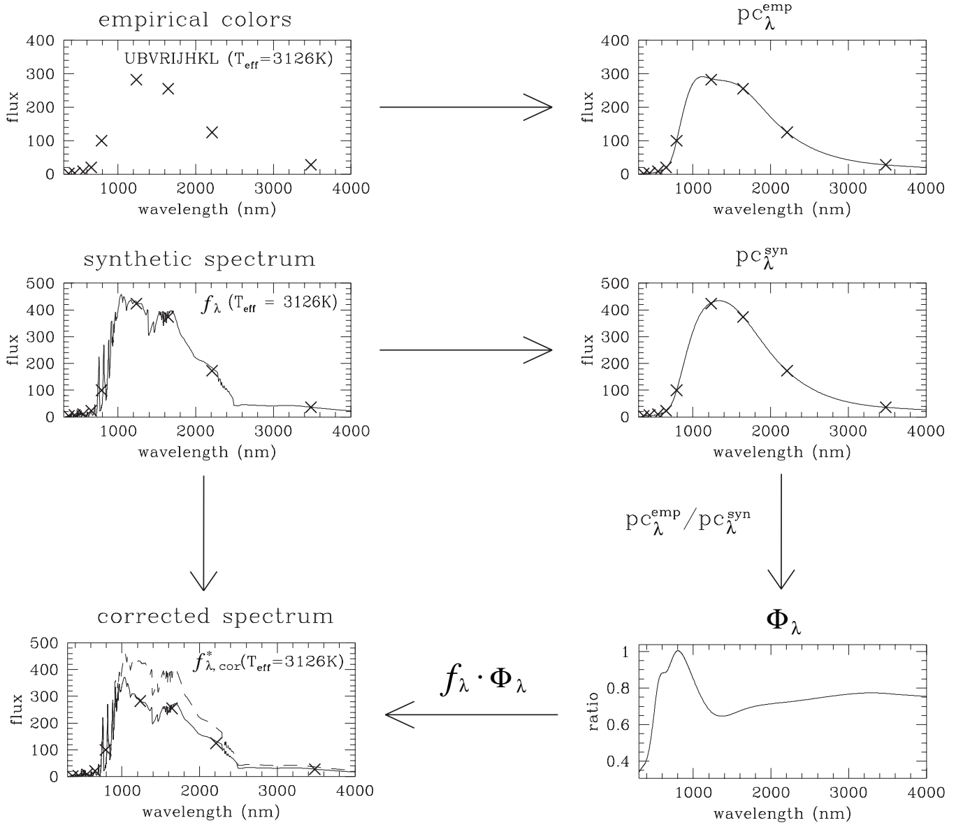
Fig. 10. Correction procedure. All fluxes are normalized to f_I = 100
