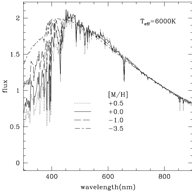
Fig. 1. K-library dwarf model spectra ( \log g = 5 ) for a range in metallicity. All the spectra are normalized at \lambda = 817 nm
