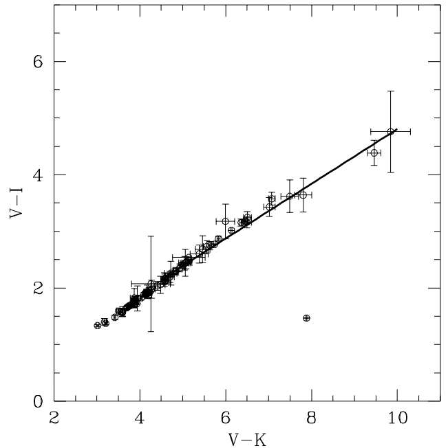
Fig. 3. Adopted (V - I) - (V - K) two-color calibration sequence for cool giants. Symbols represent mean values derived from observations given by Fluks et al. (1994). The solid line is a linear least–squares fit to the data for V - K \geq 5
