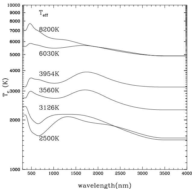
Fig. 9. Color temperatures for synthetic spectra covering a range of effective temperatures, as labelled. Top pair: K-library dwarf models; middle pair: K-library giant models; bottom pair: B + F-library giant models. Note that systematically T_c < T_{\text{eff}} , as tracked down by the black-body fit temperatures, T_{\text{mean}}
