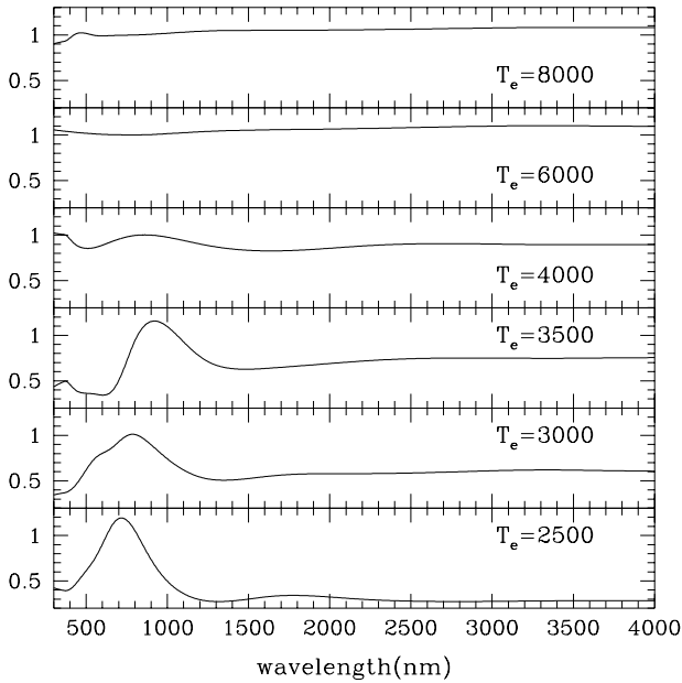
Fig. 11. Correction functions for a range of effective temperatures
