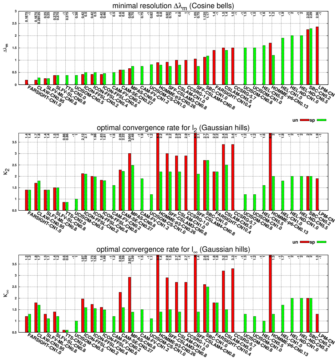
Fig. 3. Histogram of minimal resolution \Delta\lambda_m (upper), \kappa_i , i = 2, \infty , which are the “optimal” convergence rates for \ell_2 (middle) and \ell_\infty (lower), for the unlimited (“un”, red) and shape-preserving (“sp”, green) versions of the schemes. The histogram is ordered monotonically according to \Delta\lambda_m for the unlimited schemes so that \Delta\lambda decreases from left to right. For schemes for which unlimited results are not available, \Delta\lambda_m for the shape-preserving scheme is used for the purpose of ordering (schemes concerned are CAM-FV, HEL, HEL-ND, UCISOM, UCISOM-CS), and a placeholder value of -1 is used in all histograms. Note that the LPM scheme was run with fixed time step and not with a fixed Courant number; therefore no CN value is appended to the LPM label.
