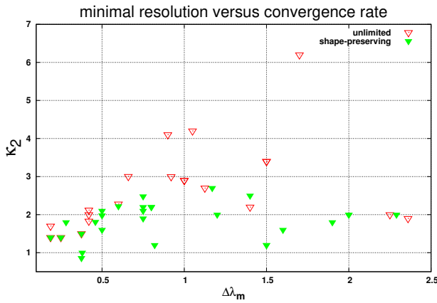
Fig. 4. “Scatter-like” plot of the data shown as histograms in Fig. 3 upper and middle rows. Each scheme is represented by a point on the plot with (x, y) coordinates (\Delta\lambda_m, \mathcal{K}_2) . For clarity each point is not labeled with a scheme acronym. The purpose of this figure is to show that there is not necessarily a correlation between “optimal” convergence rate and “minimal” resolution.
