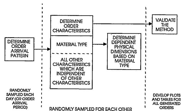
Figure 2. Steps in the Order Generation Process
