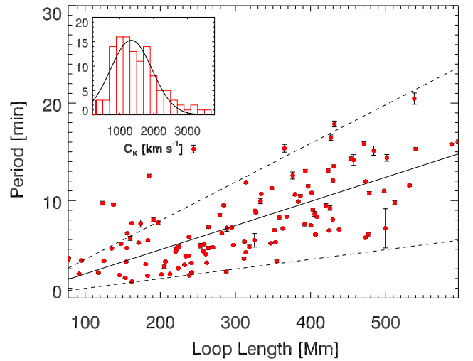
Fig. 9. Period plotted against loop length for 118 kink oscillations of coronal loops. The solid black line corresponds to an unweighted linear fit of the data. The best fitting linear function is P[\text{min}] = (0.025 \pm 0.001) L[\text{Mm}] , giving a kink speed of C_k = (1330 \pm 50) \text{ km s}^{-1} from the gradient. The dashed lines correspond to kink speeds of 800 and 3300 \text{ km s}^{-1} for the upper and lower lines, respectively.
